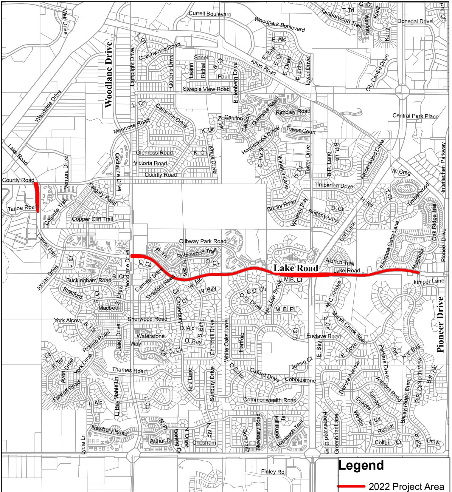
FIGURE 1 - LOCATION MAP
